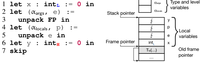
Fig. 6: Left: the value of \alpha_{\text{locals}} contains three nonsense type values, corresponding to the three variables e , p and y that has yet to enter the scope upon evaluating FP on line 3. Right: the stack layout when FP is evaluated.
